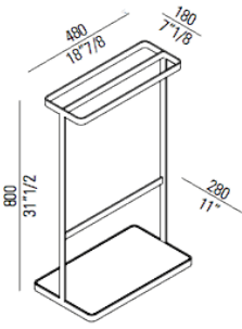
Floor towel holder AMEM862
