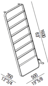
Heated towel rack AMEM871
