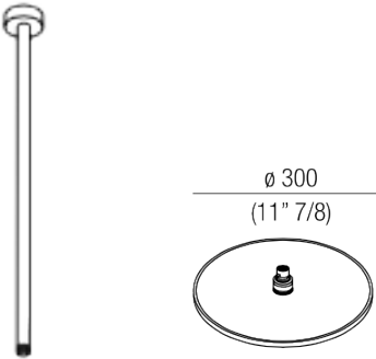
Vertical shower head pipe with Ø 300mm shower head
